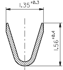
SECT. B-B (SCALE 20:1)
